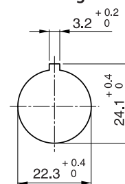
Mounting Hole
